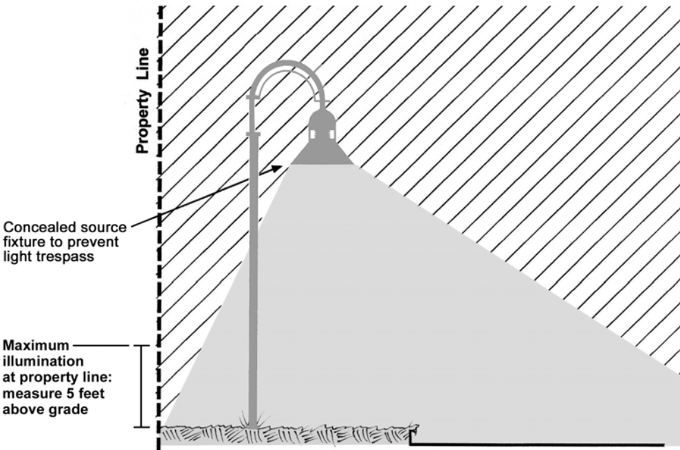
Lighting Fixture Orientation and Shielding
