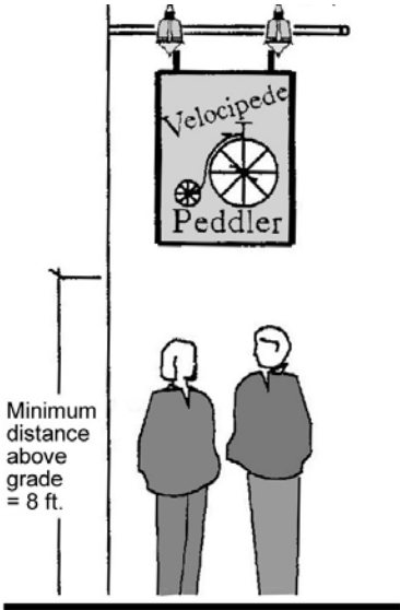
Projecting Sign Detail
