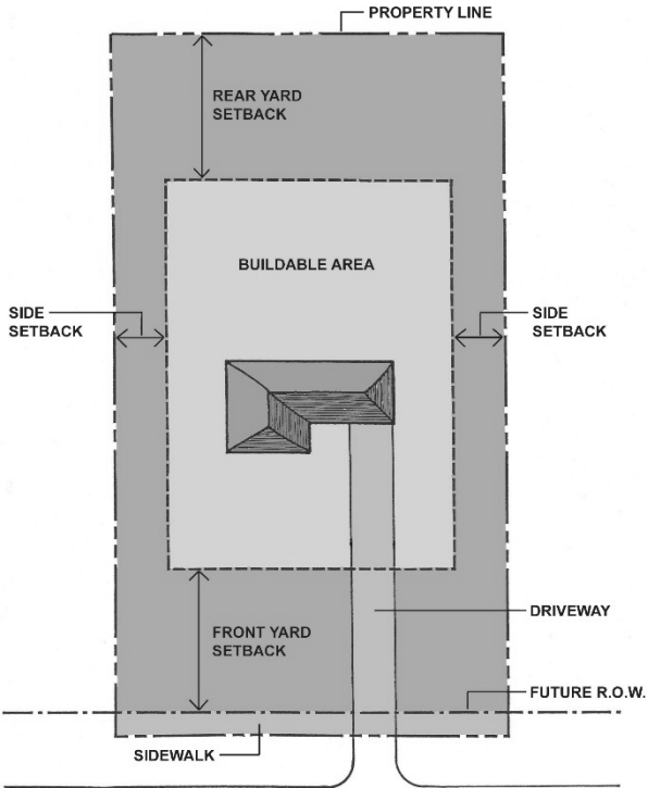
Building Envelope
