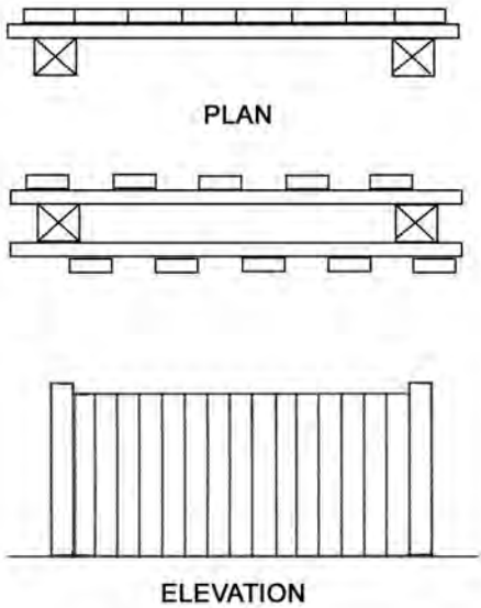
Fence
