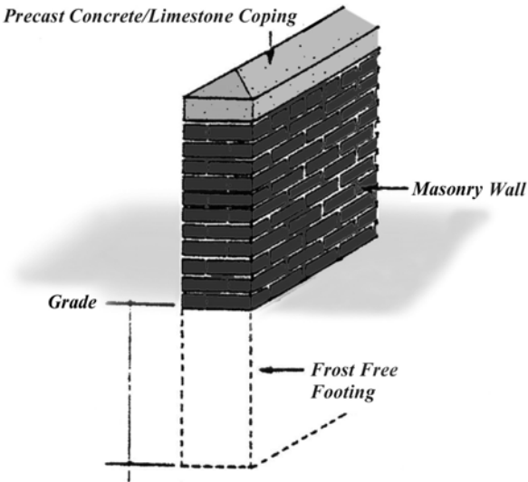
Screen Wall
